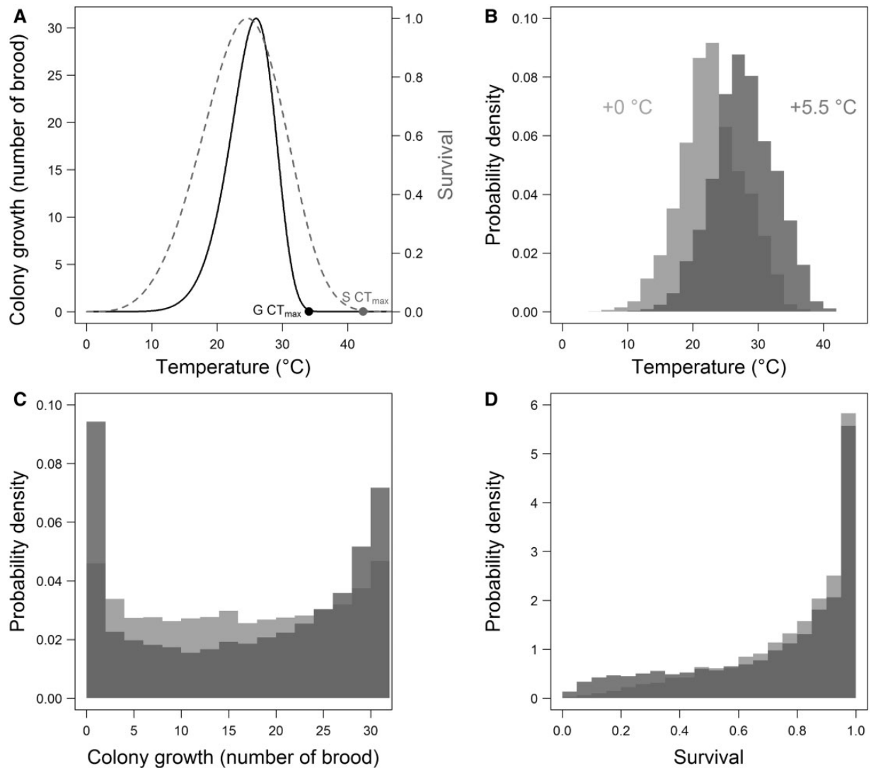
Fig. 2. Laboratory-estimated colony-growth and survival functions for T. curvispinosus in the context of air temperatures from the warming chambers. (A) Colony growth (solid line) and survival (dashed line) as functions of temperature (°C), with the estimated CT_{max} for each indicated as G CT_{max} and S CT_{max} , respectively. (B) Distributions (using kernel density estimation) of air temperatures of the +0°C and +5.5°C warming chambers. (C) Distributions (using kernel density estimation) of the colony-growth function evaluated using air temperatures of the chambers, with results from the +0°C (light gray bars) and +5.5°C (dark gray bars) chambers shown. (D) Distributions (using kernel density estimation) for the worker-survival function evaluated using air temperatures of the chambers, with results from the +0°C (light gray bars) and +5.5°C (dark gray bars) chambers shown.
